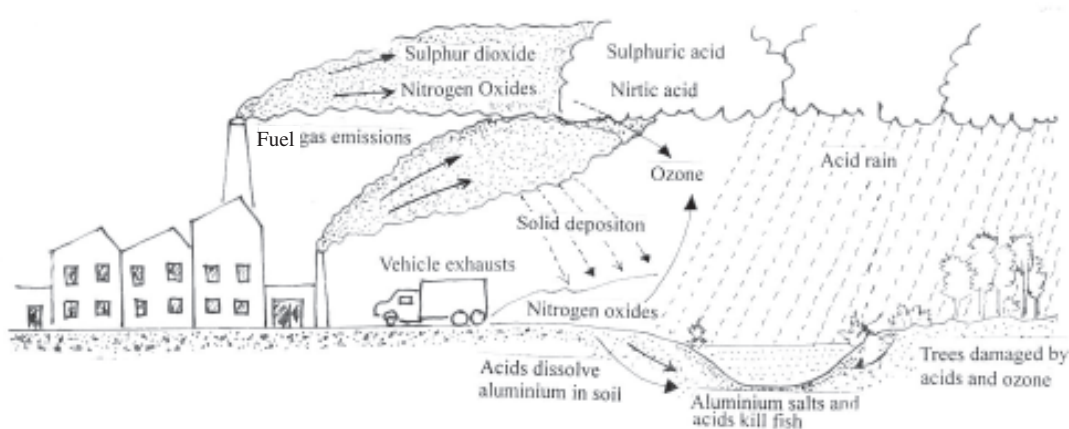
Fig.14.5: Acid rain
